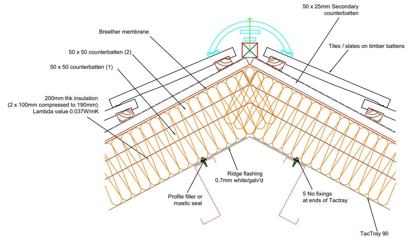
Ridge Detail
