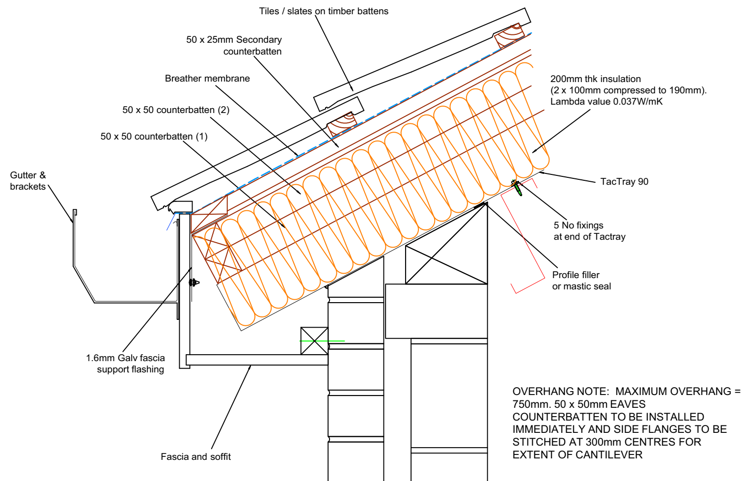
Soffited Eaves Detail
